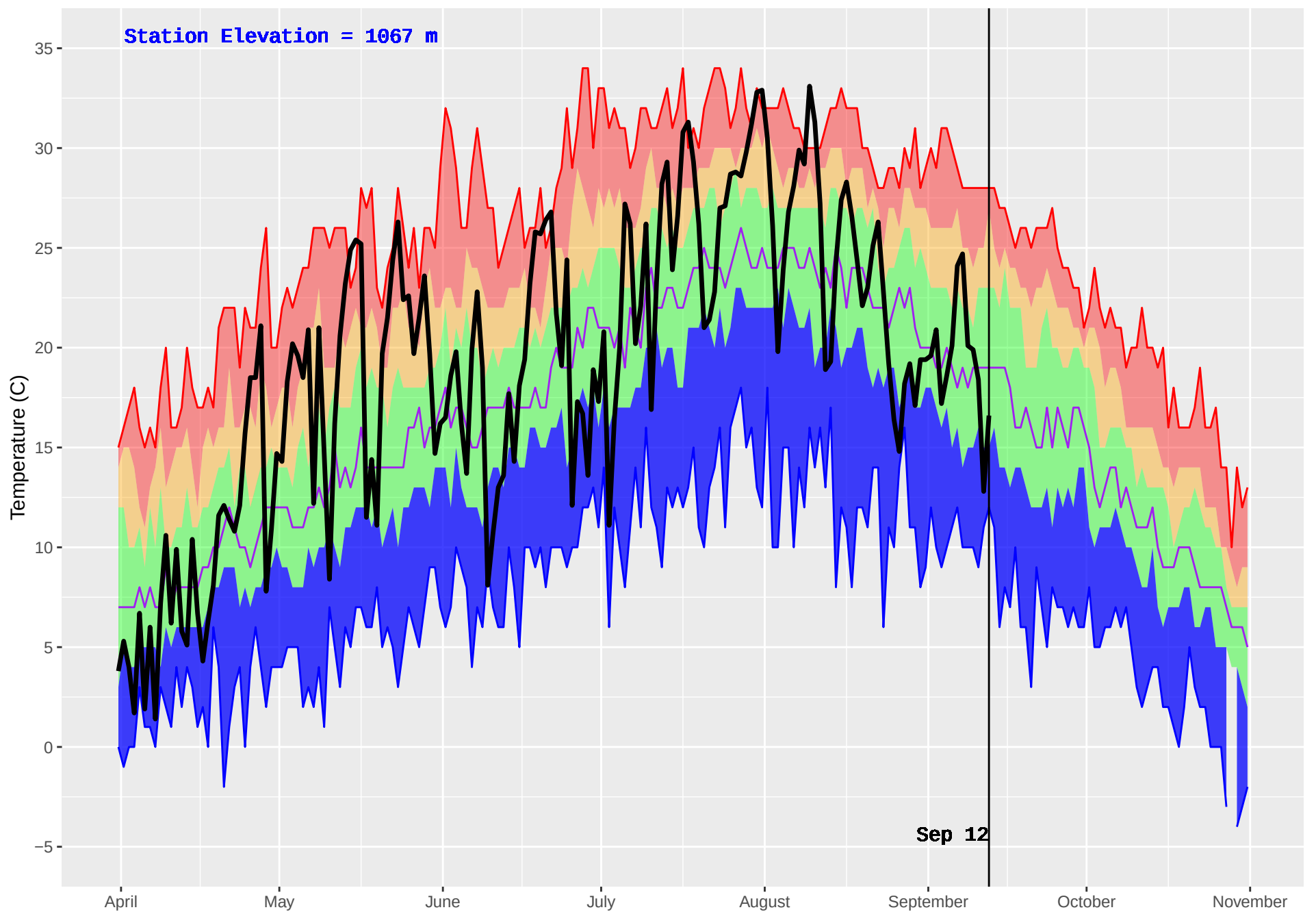
MCCUDDY (334) : Historical (1984–2016) and Current (2018) Daily Temperature
